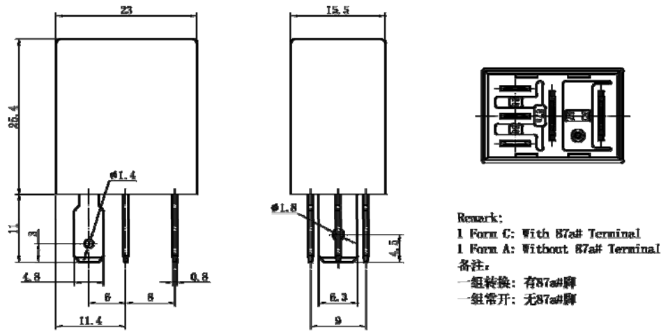
Wiring Diagram 接线图 (Bottom View 底部视图)
