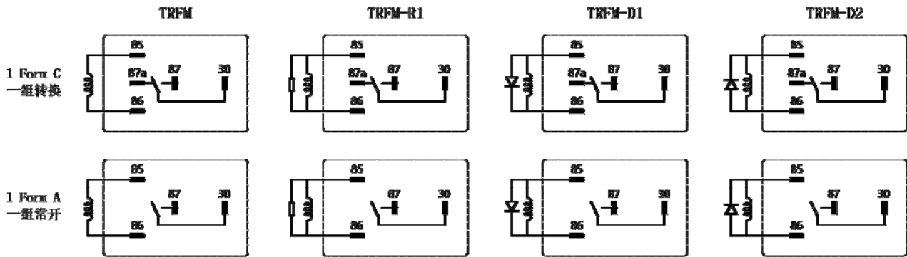
Wiring Diagram 接线图 (Bottom View 底部视图)
